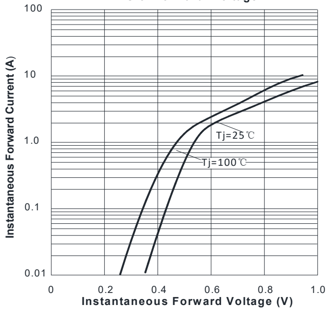
FIG.3: Forward Voltage
